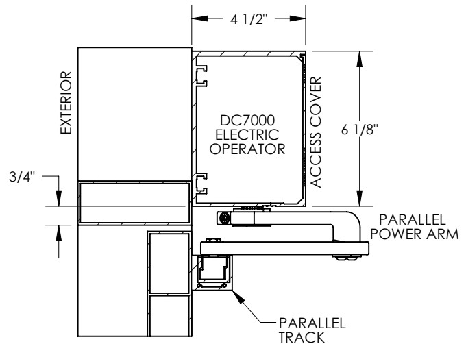
VERTICAL SECTION A-A PARALLEL ARM
