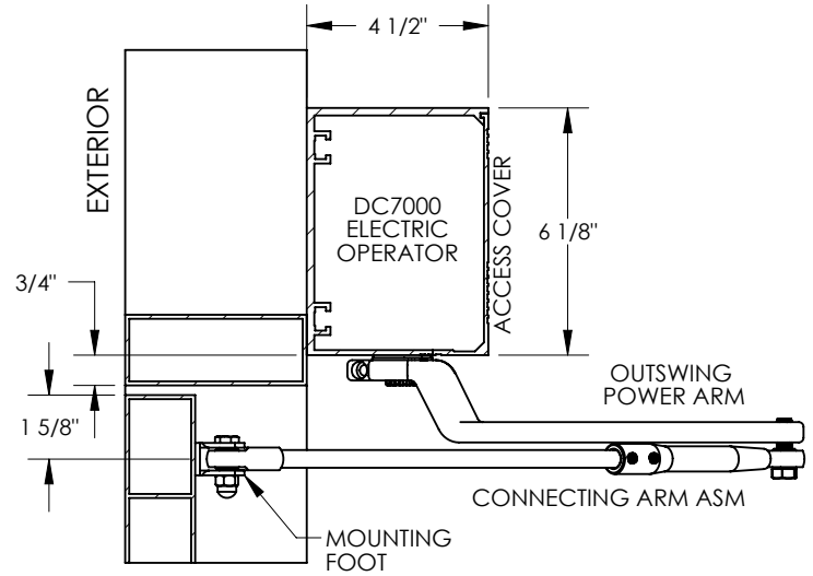
VERTICAL SECTION A-A OUTSWING ARM
