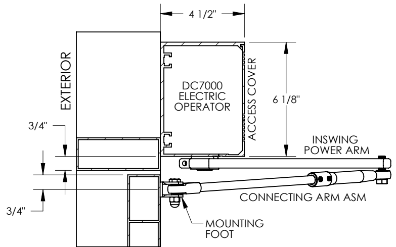
VERTICAL SECTION A-A INSWING ARM
